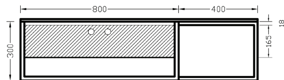
DRAWER WITH SHELF 120
